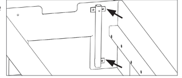
Figure F: Align outer flanges on receiver with existing holes in Reformer frame, and secure with a flat washer and nylock nut.
