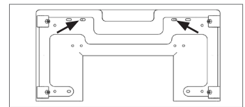
Figure R: Center Tower bracket on inner caster holes.
